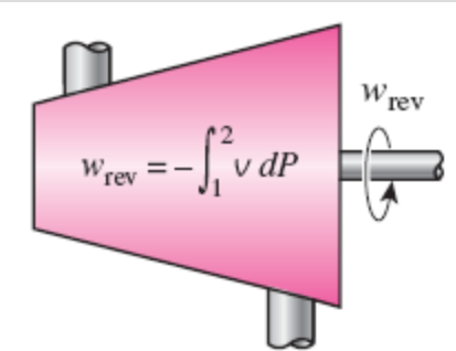
(a) Steady-flow system
